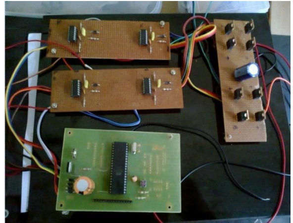
Fig. 13. 7 Level Hybrid Cascaded H-Bridge MLI.
