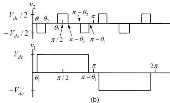
Fig. 2. H-Bridge Voltages V_1 And V_2 Which Achieve The Same Output Voltage Waveform V = V_1 + V_2 .
