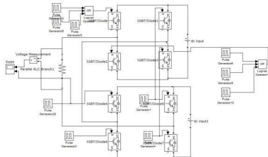
Fig. 5. Seven Level Hybrid Cascaded H-Bridge Multilevel Inverter For Single Phase Induction Motor.
