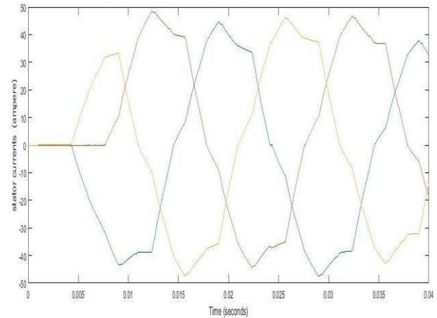
Fig. 10. Output Stator Current Waveforms For A Three Phase Circuit Connected To An Induction Motor.
